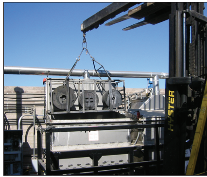
Figure 3. First set of dies removed from the cleaning tank. (At this point in time forklift was being used because overhead crane had not yet been installed.)
